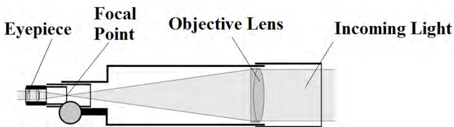
Refracting telescope cross section, WikiCommons, MesserWoland, 2006
