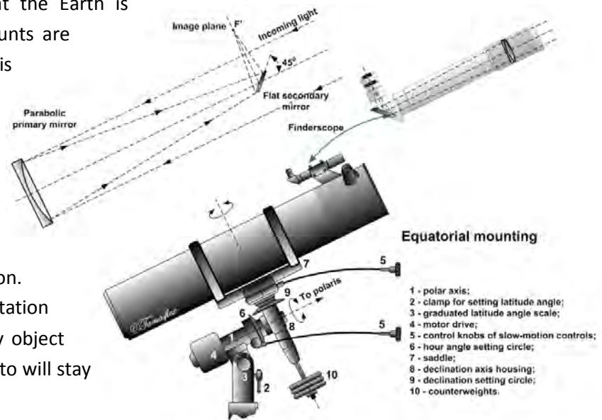
Newtonian reflector with equatorial mount, Wikipedia, Tamasflex, 2009
