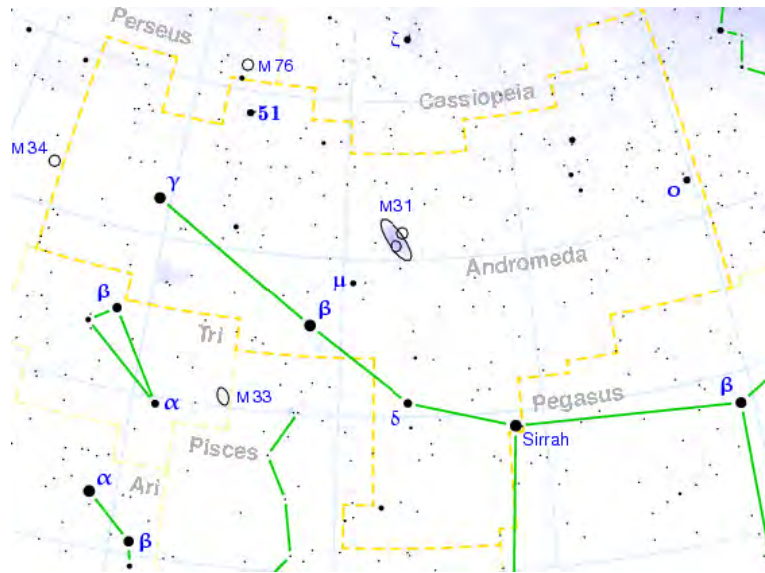
Location of M31 in Andromeda, Wikipedia, Bronger, 2005
