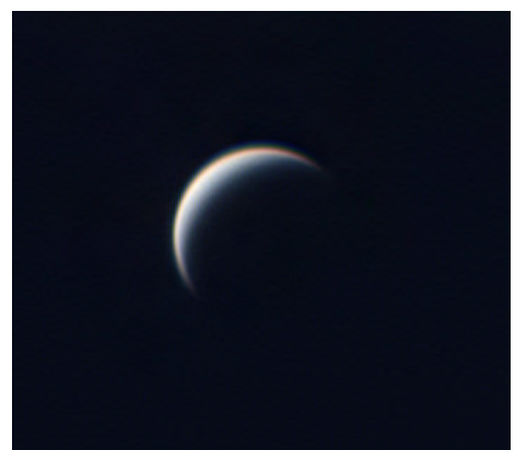
Crescent phase of Venus, Wikipedia, Marc Leclaire, 2010
