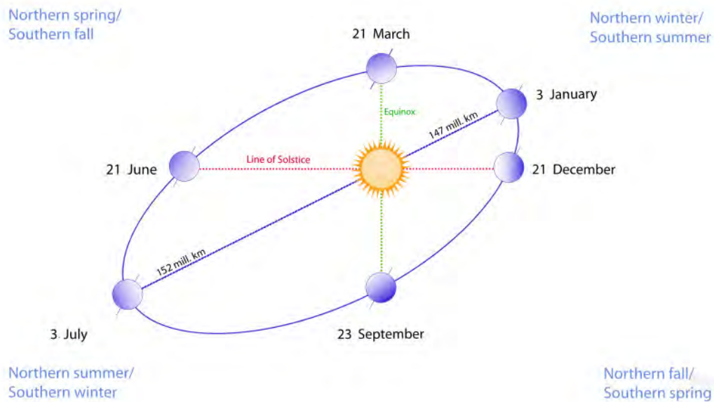
Orbit of the Earth around the Sun, Wikipedia, Gothika, 2010
