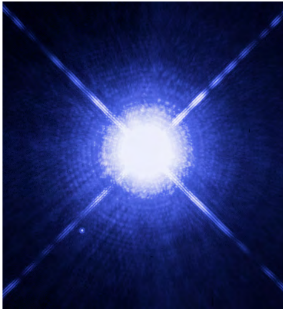
Sirius in Canis Major, Wikipedia, NASA, 2003
