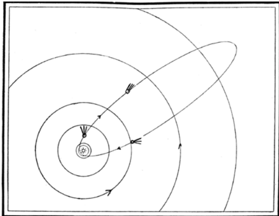
Path of Halley's Comet orbit around the Sun, Wikipedia, Popular Science Monthly, 1910
