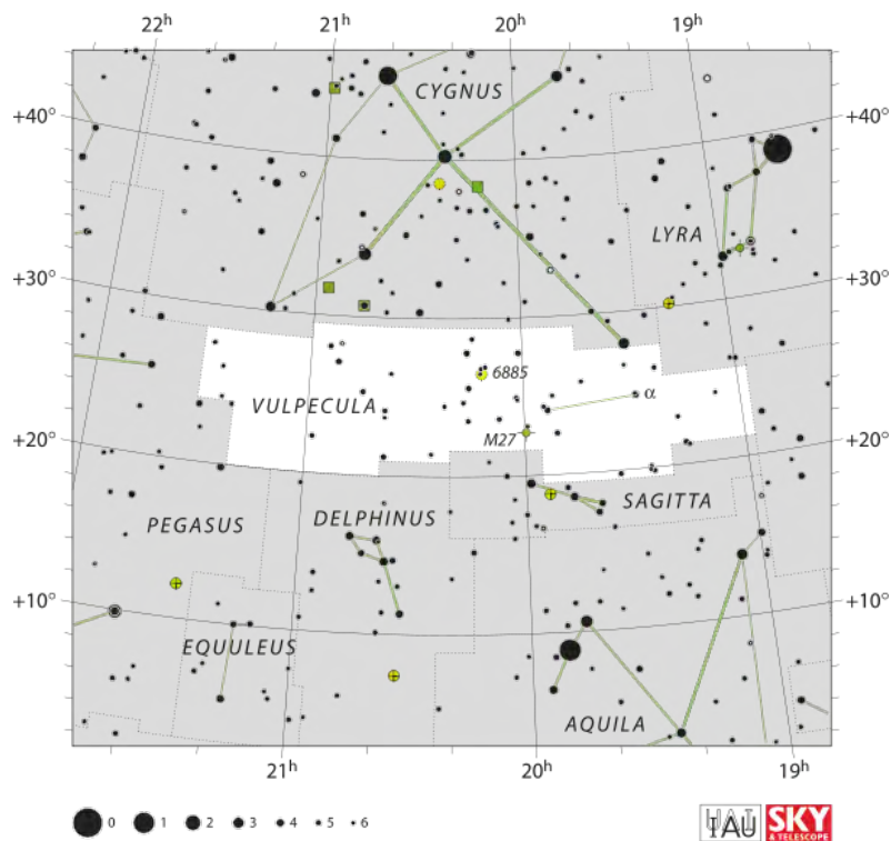
Location of M27 in Vulpecula, Wikipedia, IAU and Sky & Telescope magazine, Roger Sinnott & Rick Fienberg
