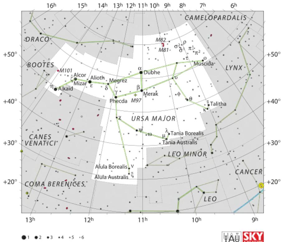
Location of M81 in Ursa Major, Wikipedia, IAU and Sky & Telescope magazine, Roger Sinnott & Rick Fienberg
