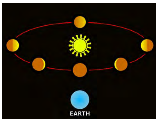
Phases of Venus, Wikipedia, Nichalp, 2006
