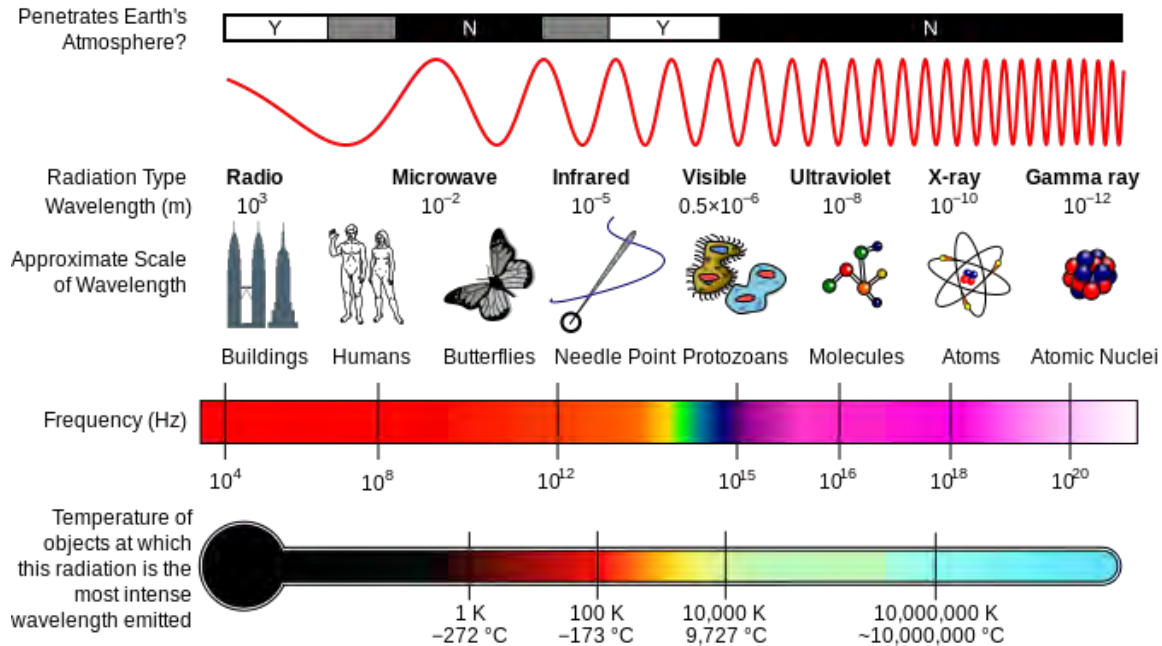
Light spectrum with relative sizes of wavelengths, Wikipedia, Inductiveload, NASA, 2007
