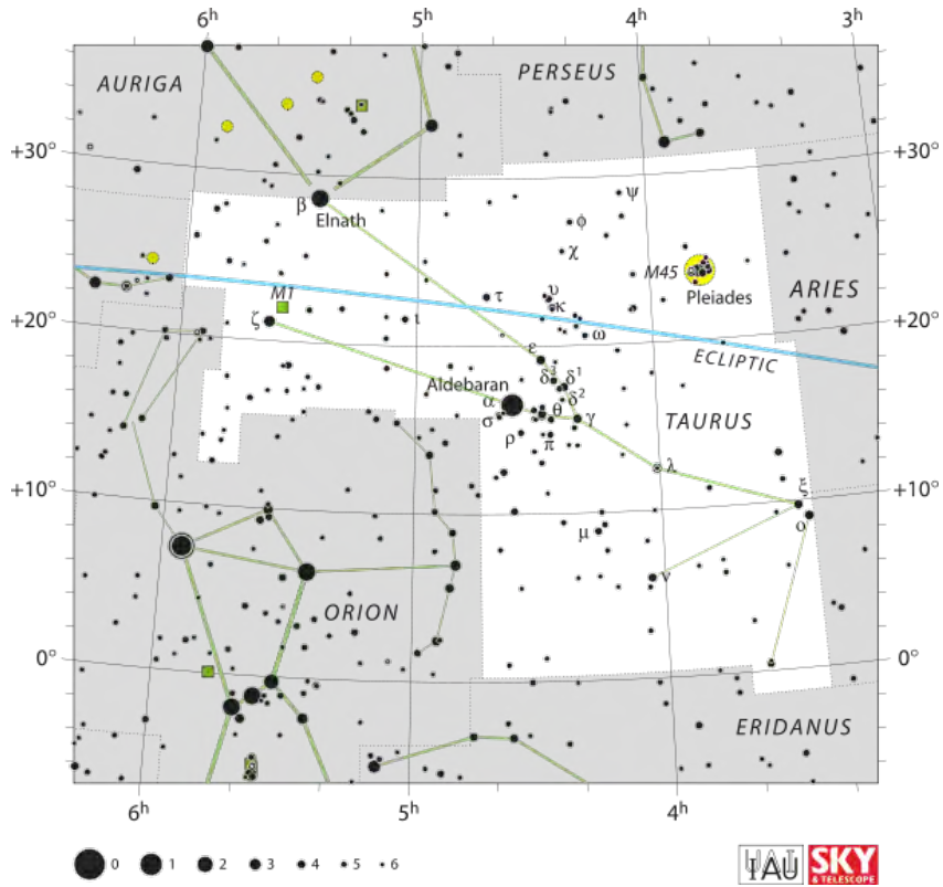
Location of M1 and M45 in Taurus, Wikipedia, IAU and Sky & Telescope magazine, Roger Sinnott & Rick Fienberg
