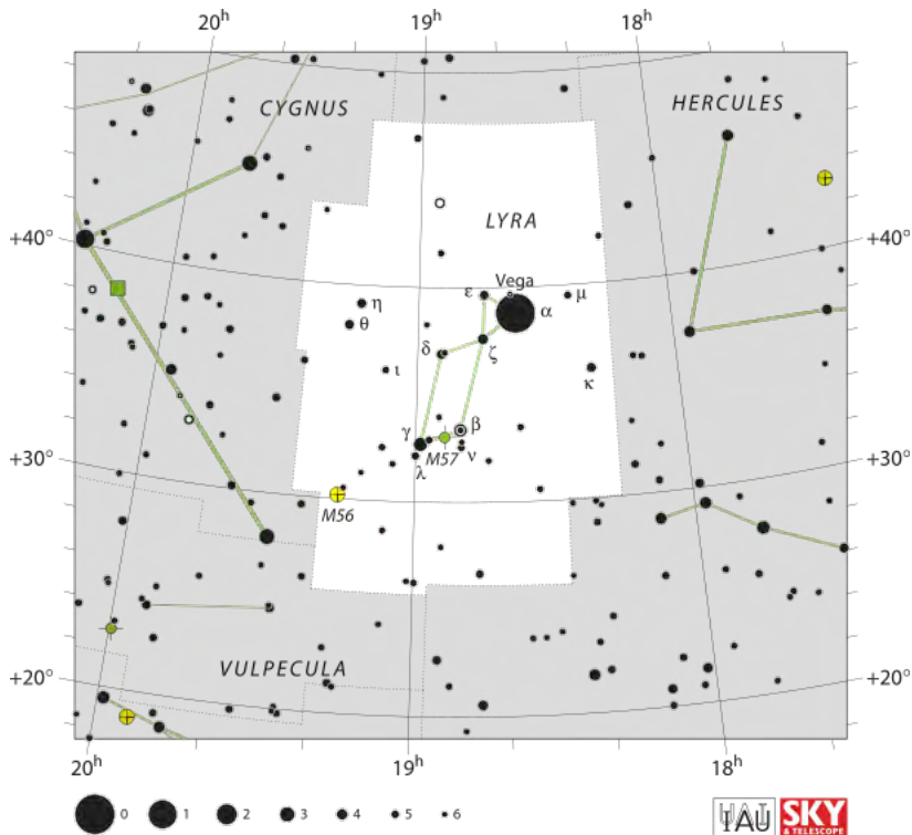
Location of M57 in Lyra, Wikipedia, IAU and Sky & Telescope magazine, Roger Sinnott & Rick Fienberg
