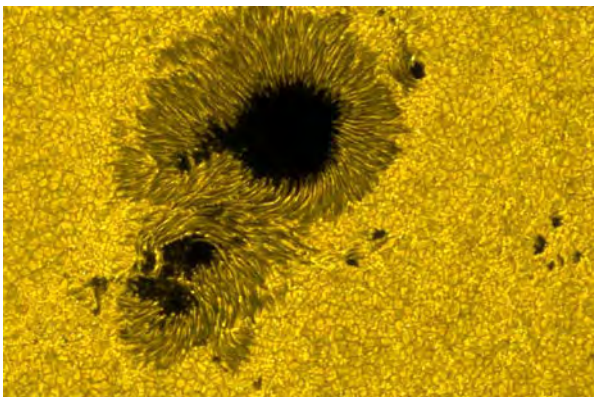
Close-up of sunspots, Wikipedia, NASA, 2006
