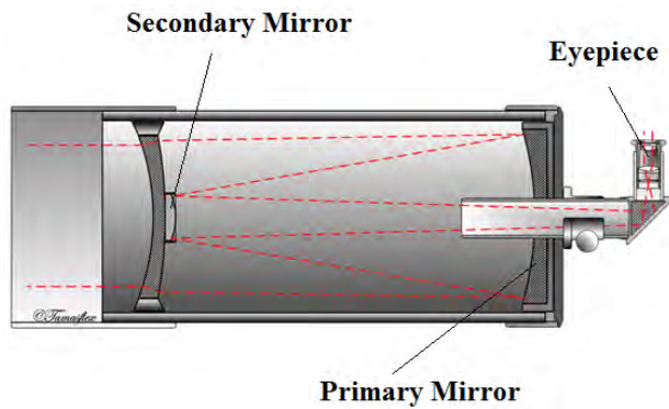
Cassegrain reflector cross section (red dotted line is incoming light), WikiCommons, Tamasflex
