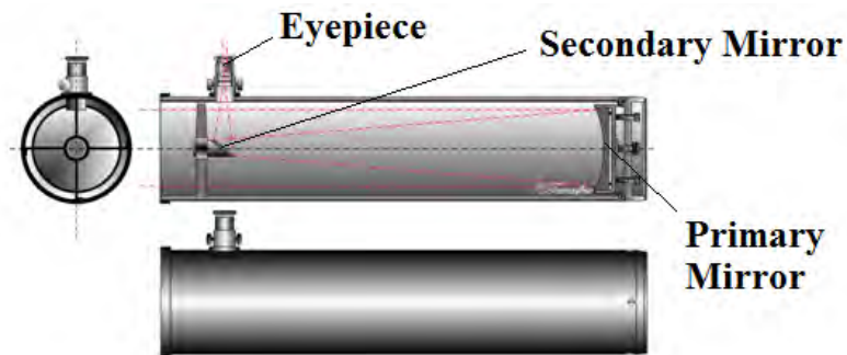
Newtonian reflector cross sections (dotted line is incoming light), Wikipedia, Tamasflex, 2009
