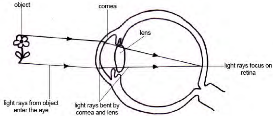
Light entering eye with lens focusing light onto retina, WikiCommons, Ruth Lawson, 2007
