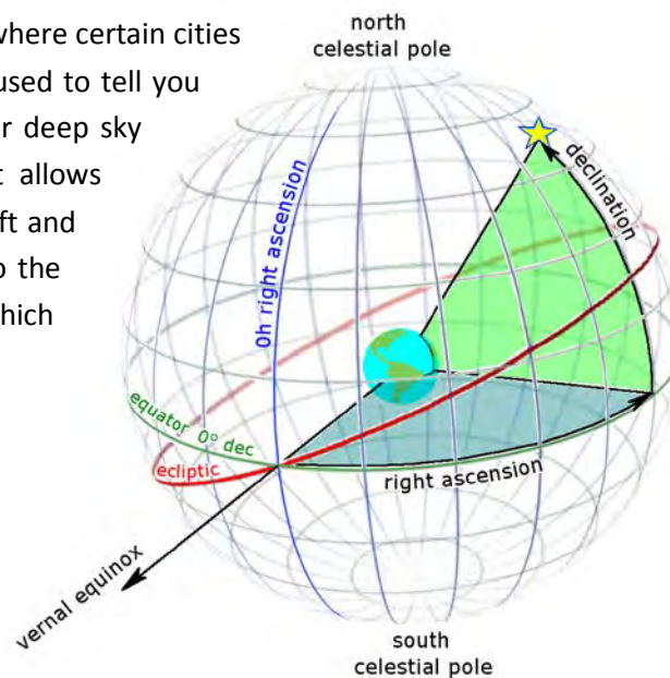
RA and Dec. coordinates, Wikipedia, Tfr000, 2012
